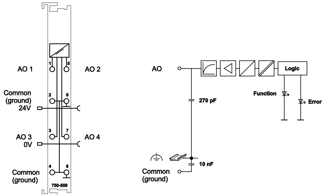
Figure 6: Schematic Diagram
