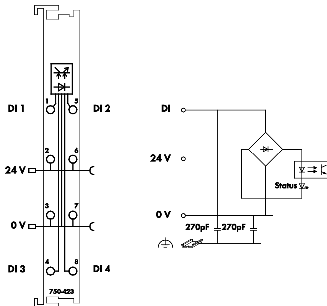
Figure 6: Schematic diagram
