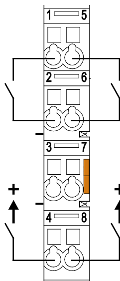
Figure 11: Connecting diagrams – 2-conductor connection
