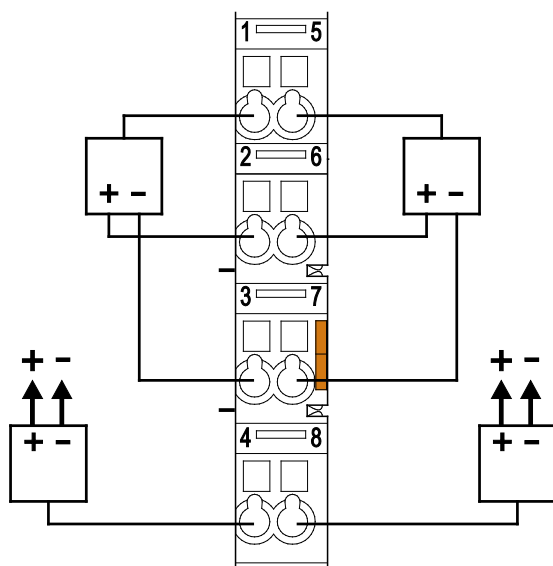
Figure 12: Connecting diagrams – 3-conductor connection
