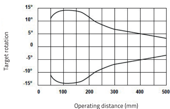
Maximum target inclination
