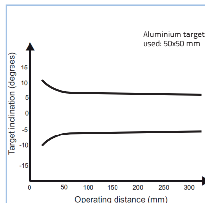
Maximum target inclination (models with analog output)
