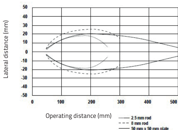
Beam - distance variation (typical values)
