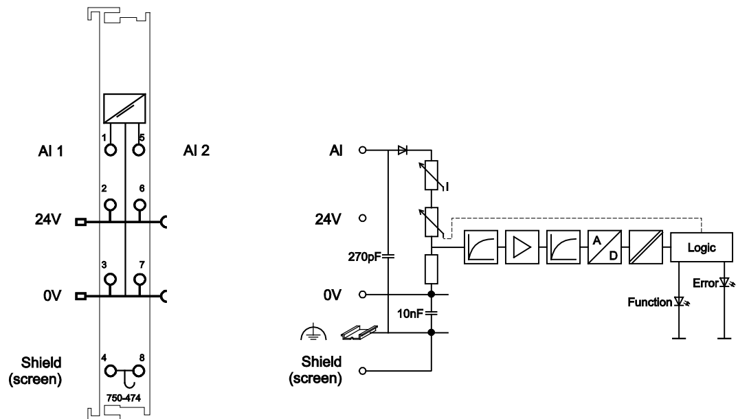
Figure 6: Schematic diagram
