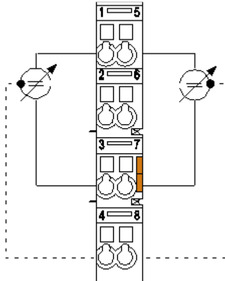
Figure 11: 2-Wire 0 V
