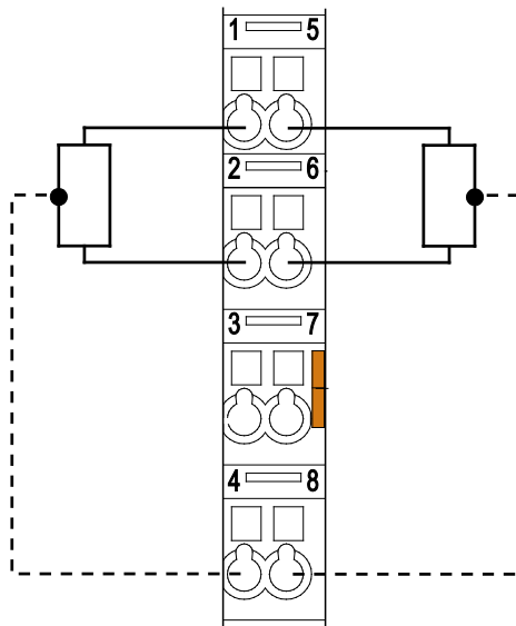
Figure 12: 2-Wire 24 V
