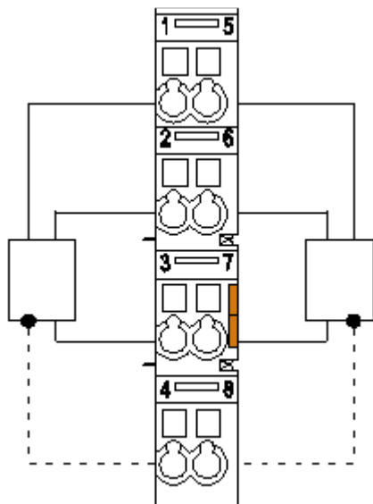
Figure 13: 3-Wire
