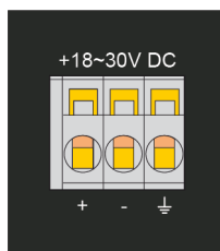
Figure 3: Power Supply (PWR) Port
