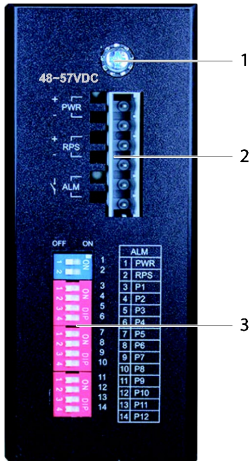
Figure 2: Top View of the industrial ECO switch
