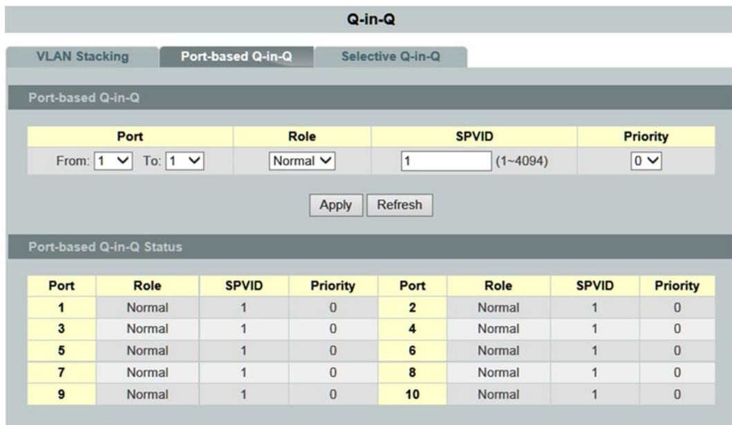
Figure 65: WBM “Q-in-Q” Page – “Port-Based Q-in-Q” Tab
