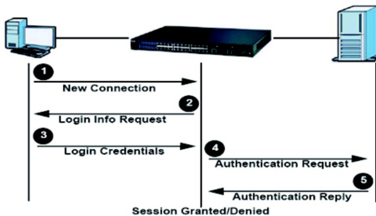
Figure 26: RADIUS Server
