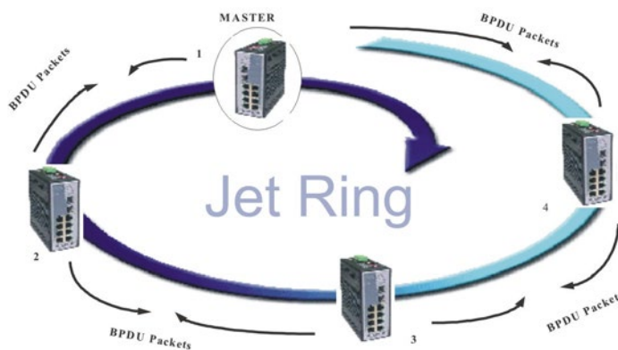
Figure 23: Jet Ring
