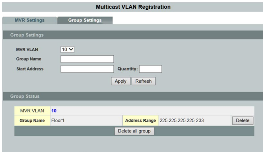
Figure 52: WBM “Multicast VLAN” Page – “Group Settings” Tab
