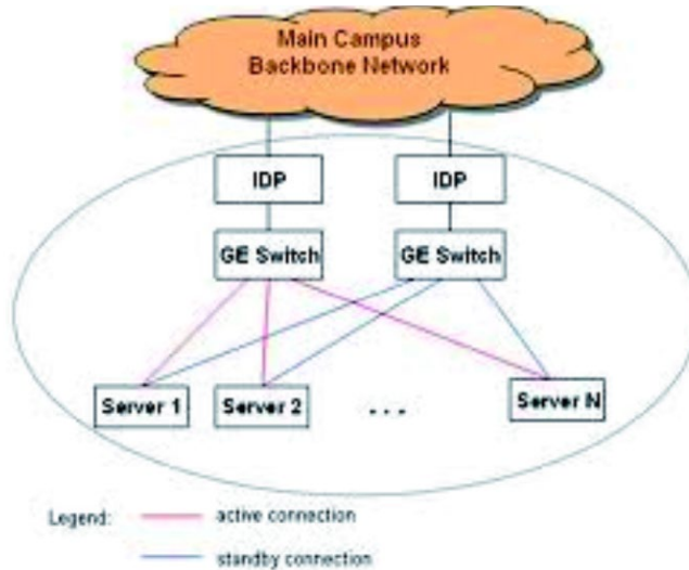
Figure 22: Dual Homing
