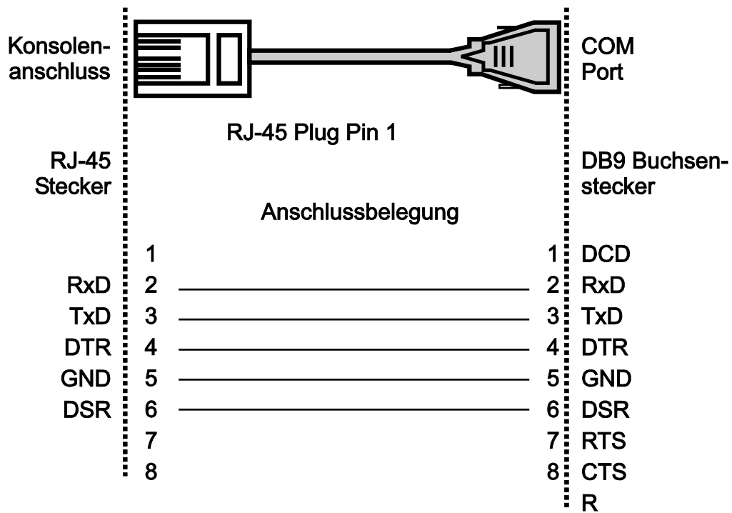
Figure 123: Connector Pin Assignment RJ-45 to DB9
