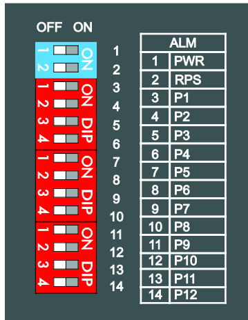
Figure 7: DIP Switches
