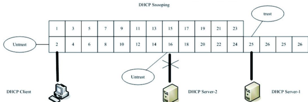
Figure 24: DHCP Snooping
