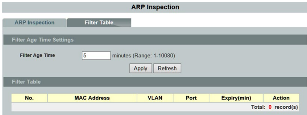
Figure 95: WBM “ARP Inspection” Page – “Filter Table” Tab
