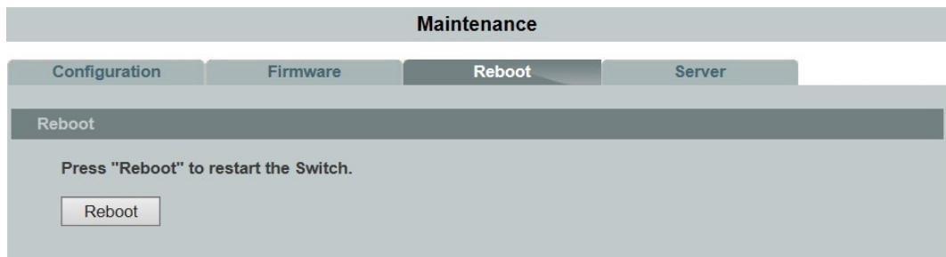
Figure 117: WBM "Maintenance" Page – "Reboot" Tab
