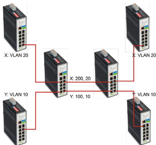
Figure 16: Port-Based Q-in-Q
