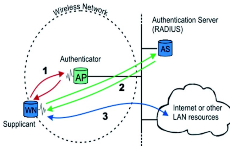
Figure 25: IEEE 802.1X
