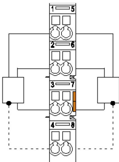
Figure 13: 3-Wire
