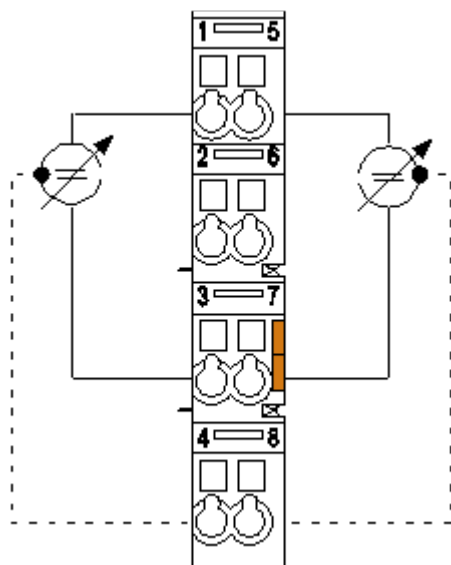
Figure 11: 2-Wire 0 V
