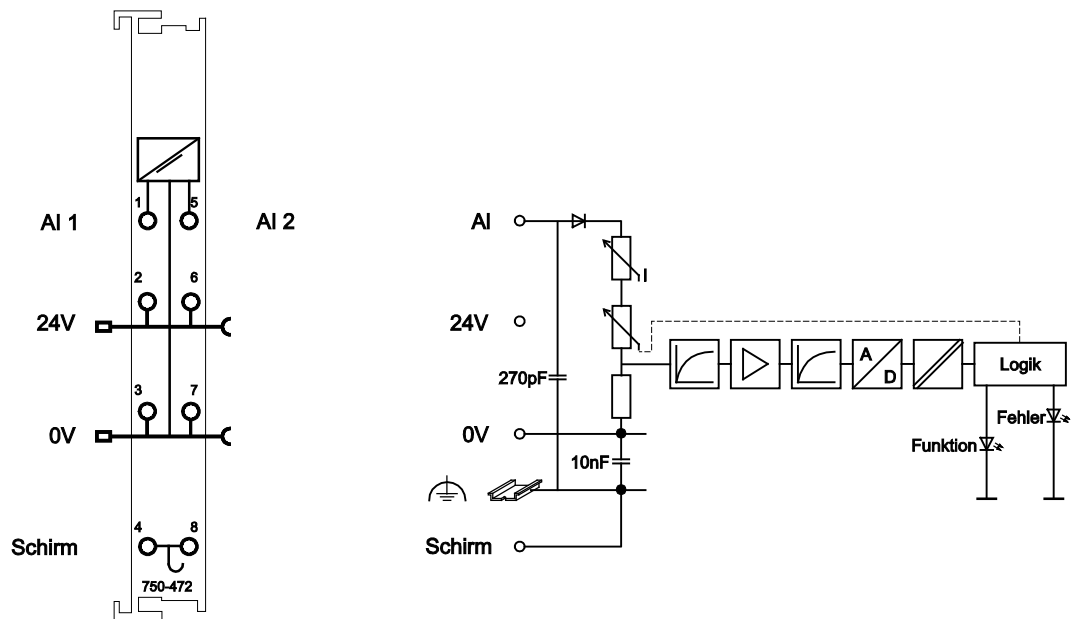
Figure 6: Schematic diagram
