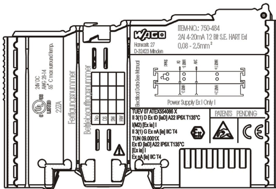
Figure 11: Side Marking Example for Ex i and IEC Ex i Approved I/O Modules According to CENELEC and IEC
