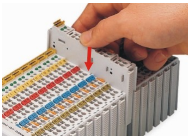
Figure 7: Snap the I/O Module into Place (Example)
