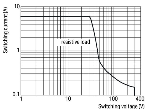
DC load limit curve
