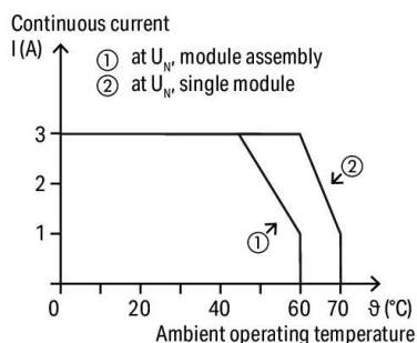
Current-carrying capacity curve
