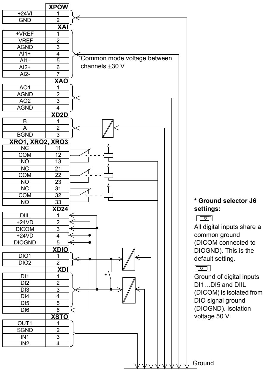
Ground isolation diagram
