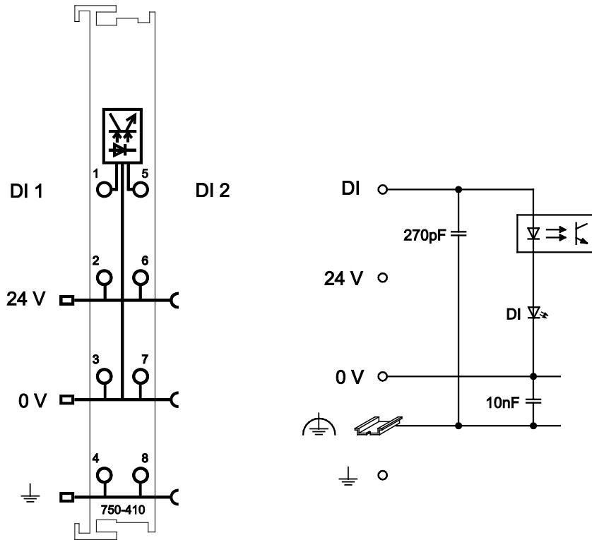
Figure 6: Schematic Diagram
