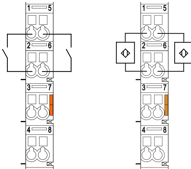
Figure 11: Connecting Diagrams, 2-Conductor Connection
