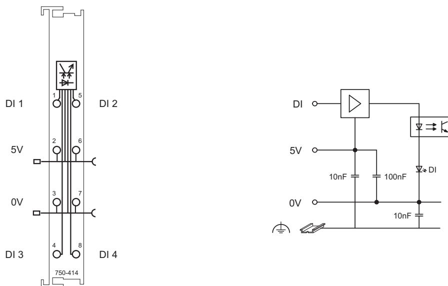
Fig. 2.1.1-3: Schematic Diagram
