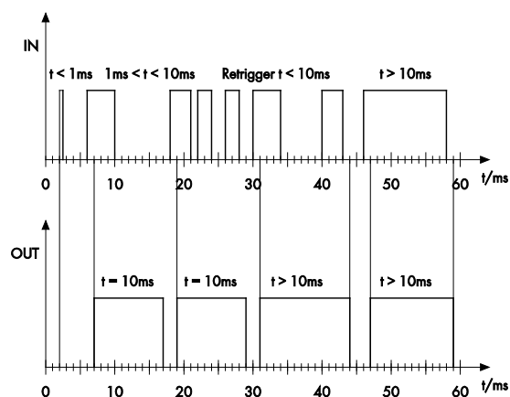
Figure 1: Pulse Extension of the input signals
