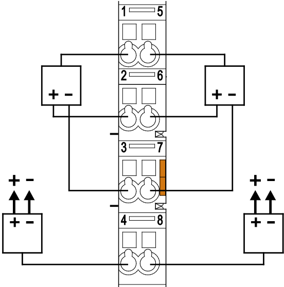
Figure 13: Connecting diagrams – 3-conductor connection
