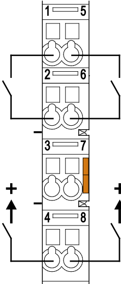
Figure 12: Connecting diagrams – 2-conductor connection
