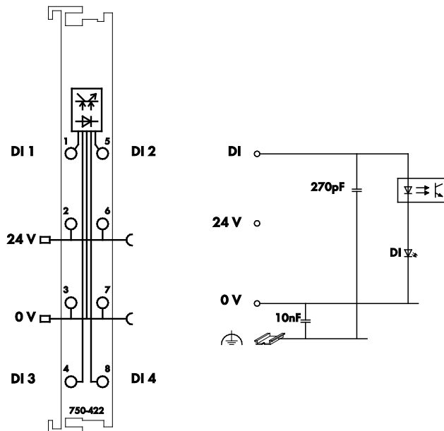
Figure 7: Schematic diagram
