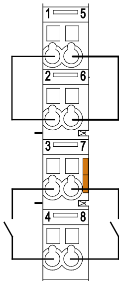
Figure 12: Connecting diagrams –2 Channels, Low-Side Switching
