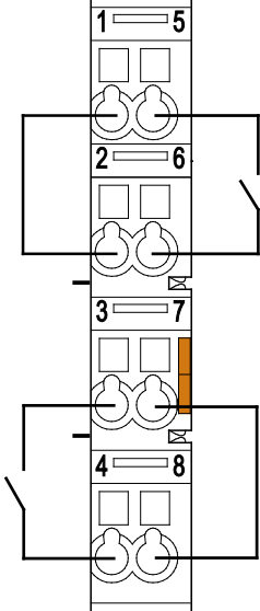
Figure 13: Connecting diagrams – 1 Channel High-Side Switching, 1 Channel Low-Side Switching
