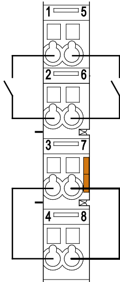
Figure 11: Connecting diagrams –2 Channels, High-Side Switching
