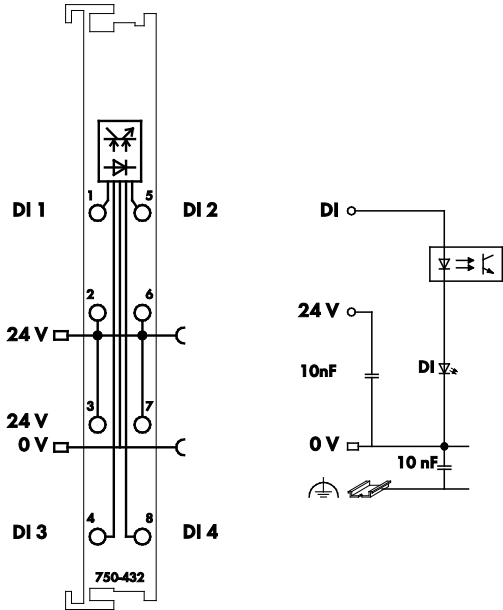
Figure 6: Schematic diagram
