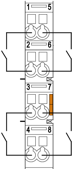
Figure 11: Connecting Diagram
