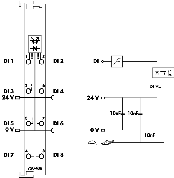
Figure 6: Schematic Diagram
