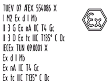
Figure 12: Text Detail – Marking Example for Approved I/O Modules According to ATEX and IECEx.
