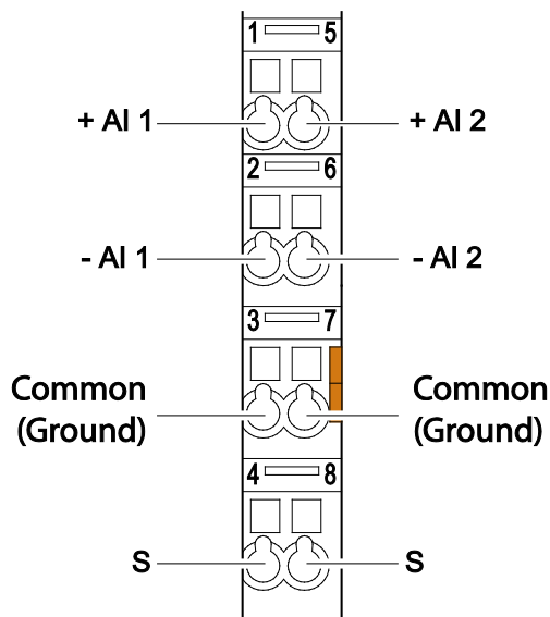
Figure 3: CAGE CLAMP® Connectors
