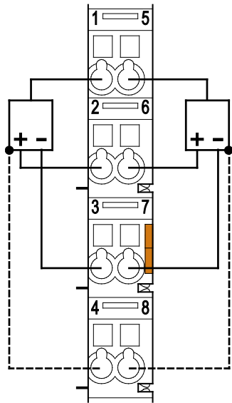
Figure 14: Connecting Diagram, 3-Conductor Connection, Grounded
