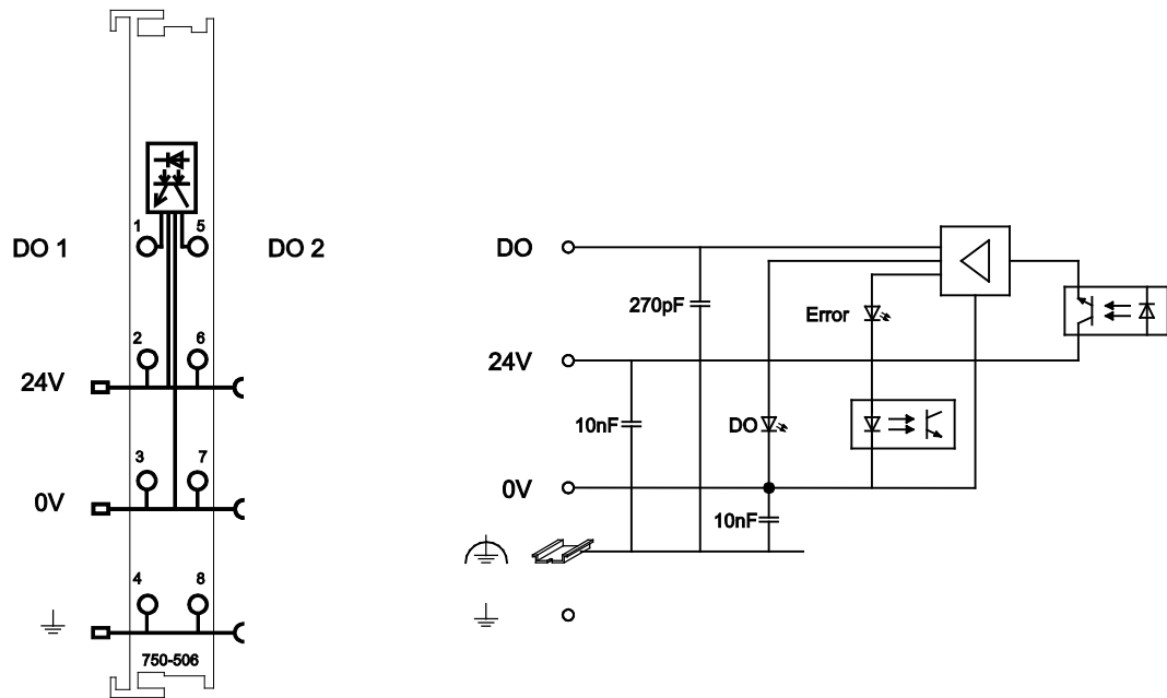
Figure 6: Schematic Diagram
