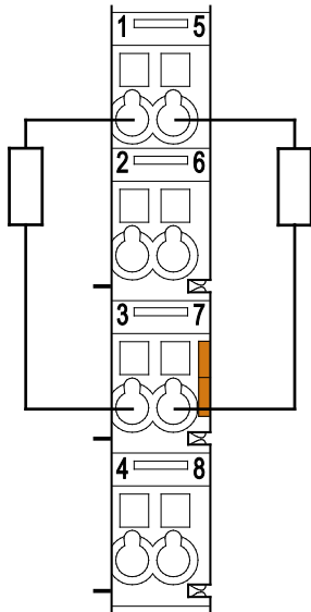
Figure 11: Connecting Diagram, 2-Conductor Connection, Ungrounded
