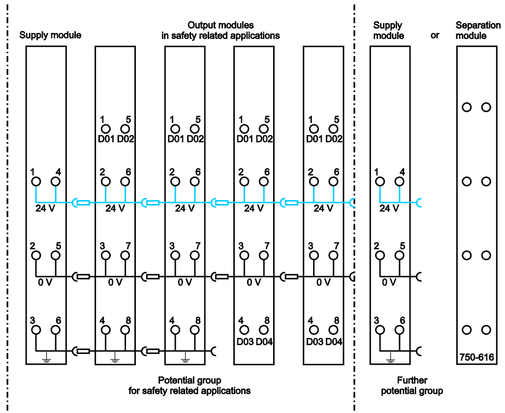
Figure 15: Potential Group for Safety Related Applications
