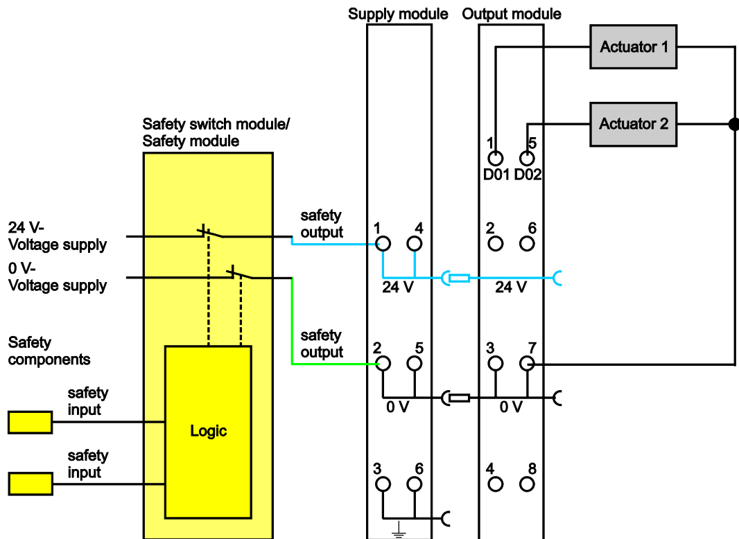
Figure 17: Two-channel Double-pole Disconnection
