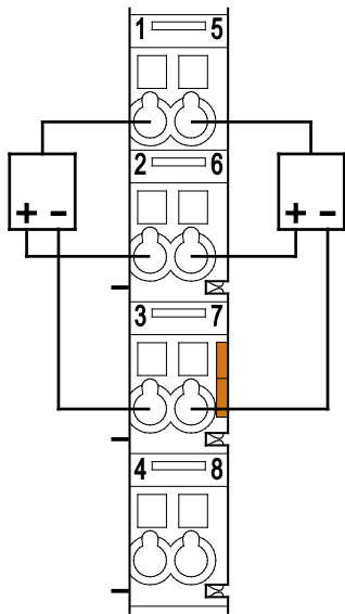
Figure 13: Connecting Diagram, 3-Conductor Connection, Ungrounded
