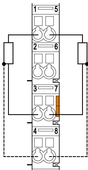
Figure 12: Connecting Diagram, 2-Conductor Connection, Grounded
