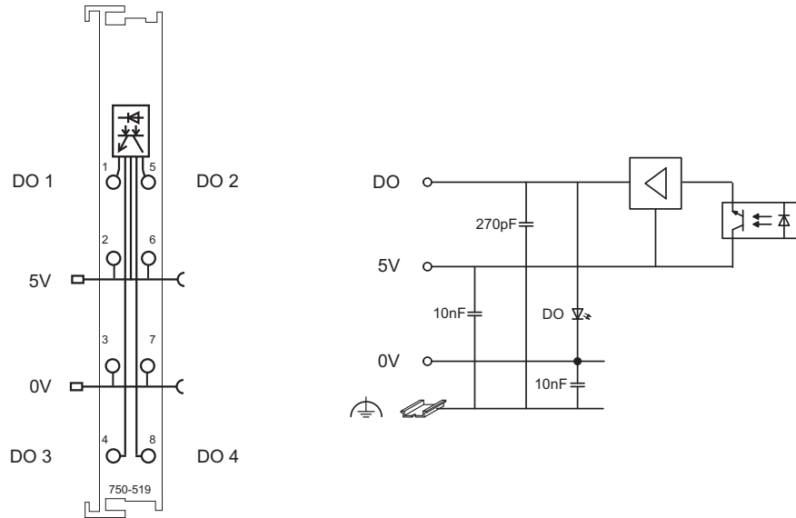
Fig. 2.1.1-3: Schematic Diagram
