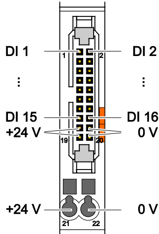
Figure 3: Connectors
