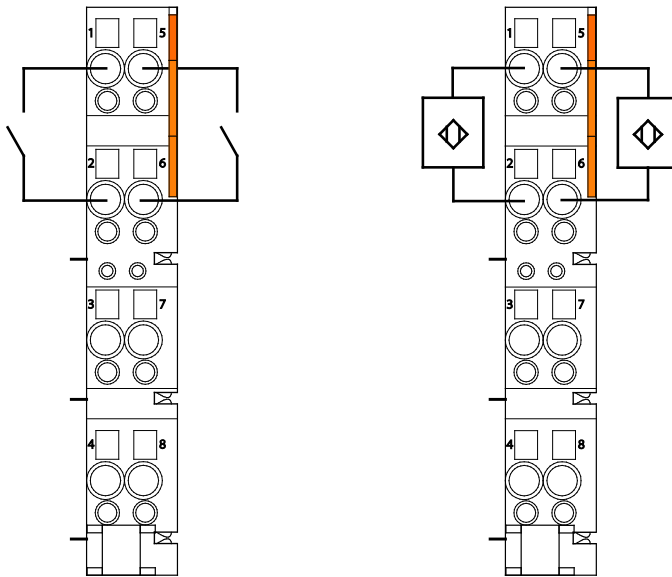
Figure 21: Connecting Diagram, 2-Conductor Connection
