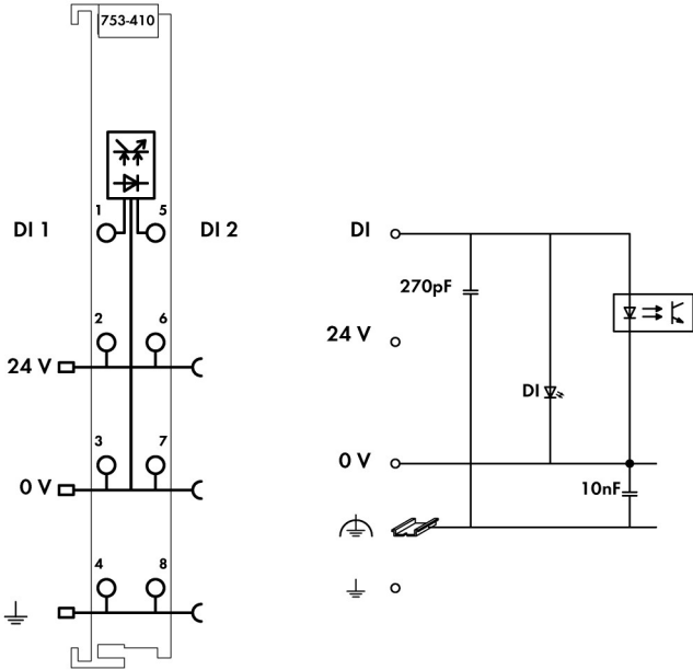
Figure 6: Schematic Diagram
