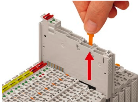
Figure 8: Removing the I/O Module (Example)
