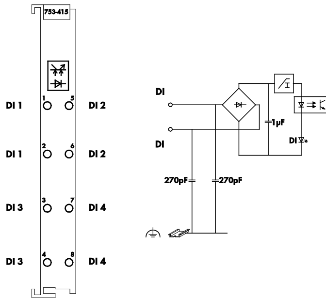
Figure 5: Schematic Diagram
