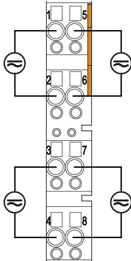
Figure 20: Connecting Diagram – 2-Conductor Connection
