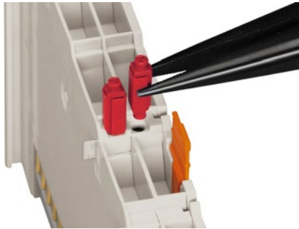
Figure 13: Inserting the Coding Fingers
