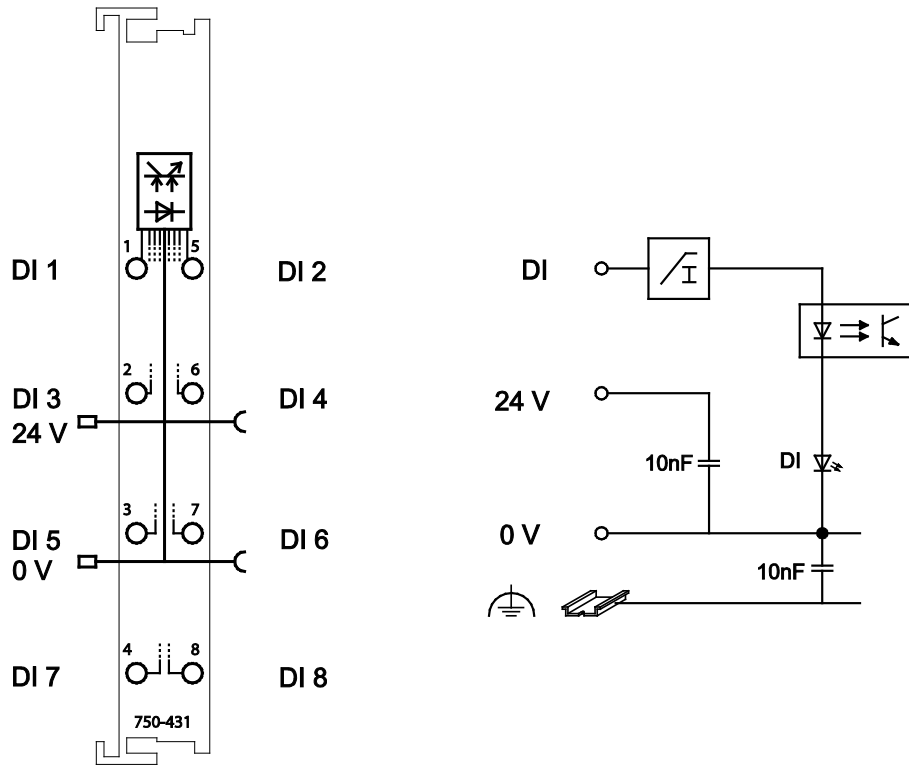
Figure 6: Schematic Diagram
