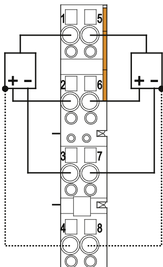
Figure 24: Connecting Diagram, 3-Conductor Connection, Grounded
