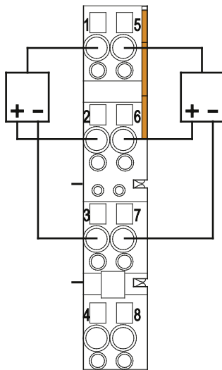
Figure 23: Connecting Diagram, 3-Conductor Connection, Ungrounded
