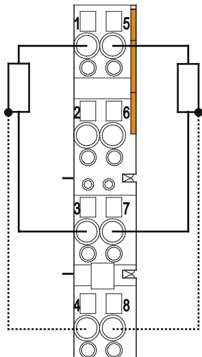
Figure 22: Connecting Diagram, 2-Conductor Connection, Grounded
