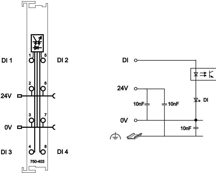
Figure 6: Schematic diagram
