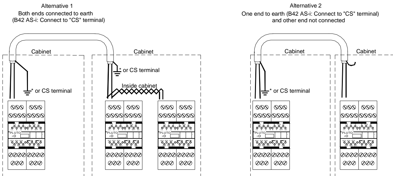
Alternatives for connection of bus cable shield *For B42 AS-i and D45 connect shield to the "CS" terminal
