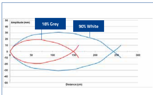
Diffused proximity
