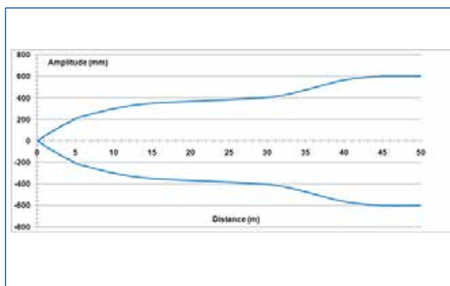
Through beam
