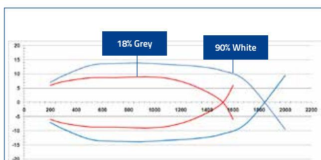
Diffused proximity
